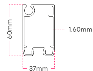
4 Narrow beam 37X60 with LED strip slot
