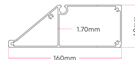
3 Wide beam 160X60
