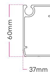
5 Narrow beam 37X60
