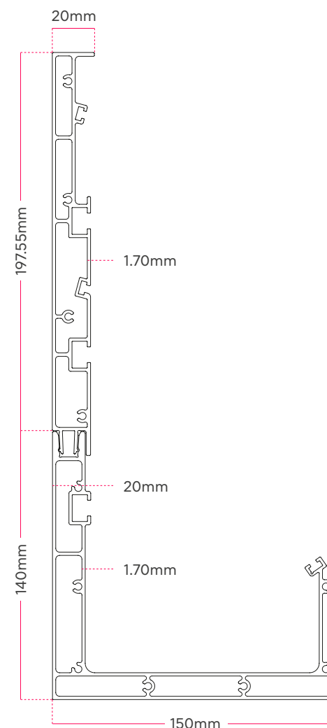
1 Perimeter frame with gutter 150X337
