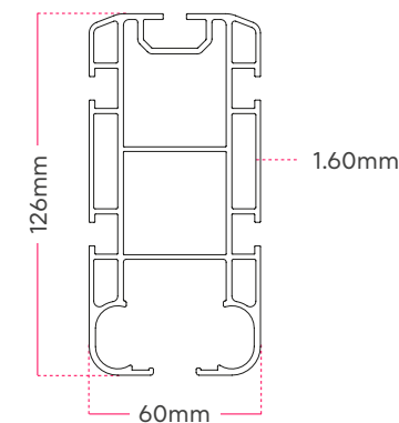
2 Rafter 60X126
